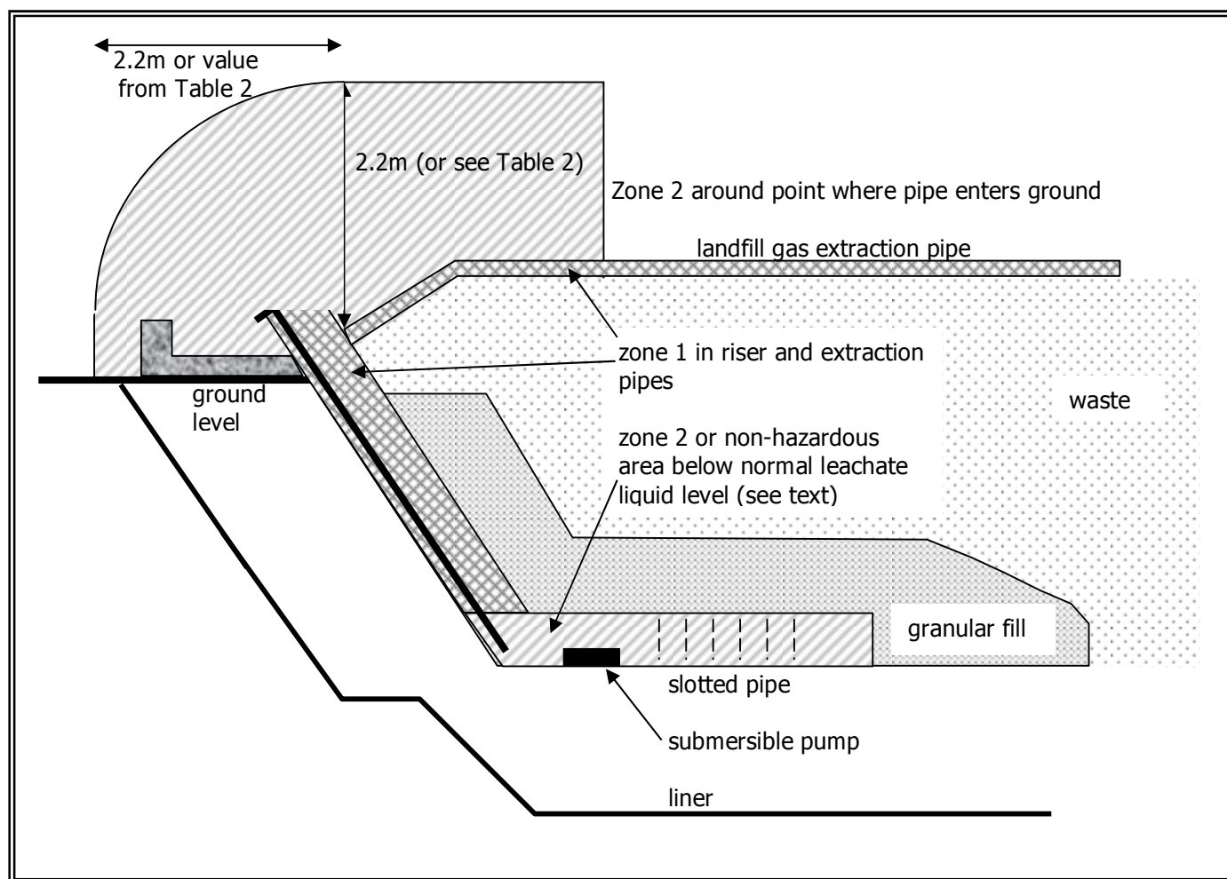
Figure 4: zoning for a leachate riser
