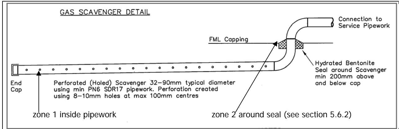
Figure 3: zoning for a typical gas scavenger pipe
