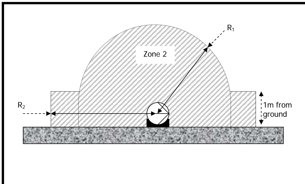
Figure 8: zoning diagram of a booster pump - outdoors
